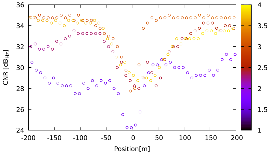
CNR vs position for G09 (L5) on SamsungS20 - DOY 263 jam. 1
