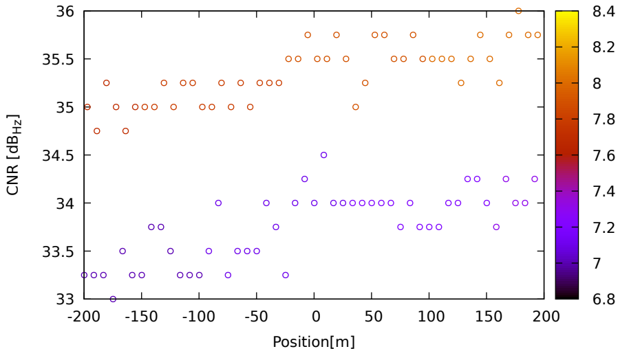
CNR vs position for G09 (L5) on SamsungS20 - DOY 263 jam. 3
