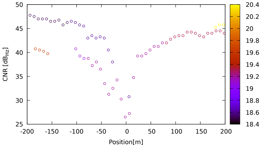
CNR vs position for G19 (L1) on SamsungS20 - DOY 263 jam. 2
