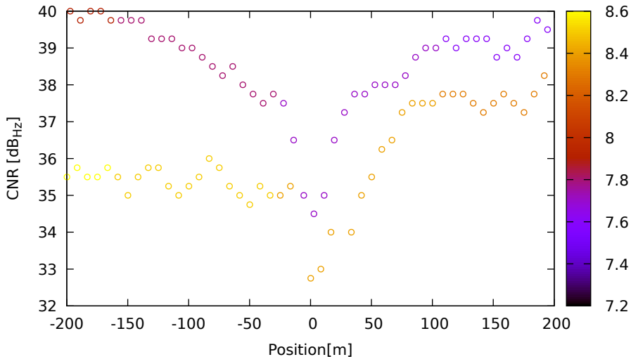
CNR vs position for G32 (L1) on SamsungS20 - DOY 263 jam. 3
