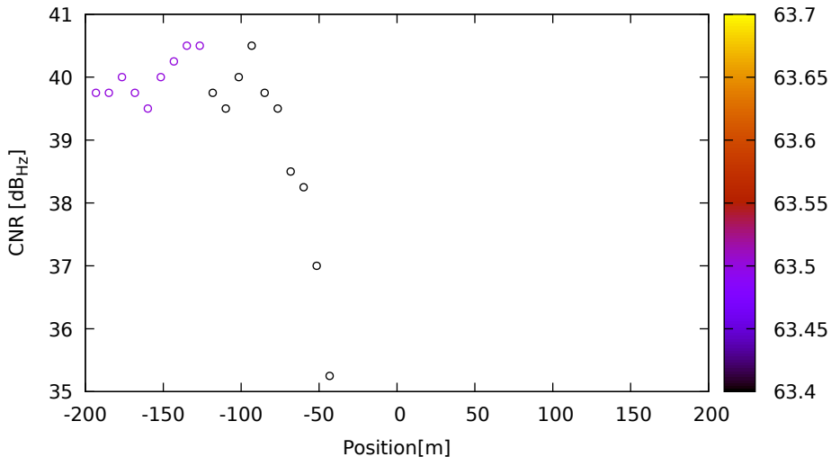
CNR vs position for R01 (G1) on SamsungS20 - DOY 263 jam. 1
