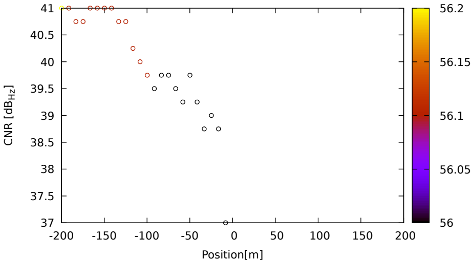
CNR vs position for R01 (G1) on SamsungS20 - DOY 263 jam. 3
