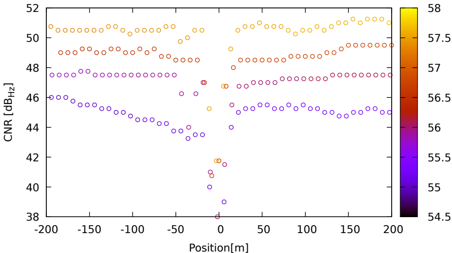
CNR vs position for R02 (G1) on SamsungS20 - DOY 263 jam. 2
