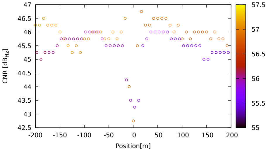
CNR vs position for R24 (G1) on SamsungS20 - DOY 263 jam. 3
