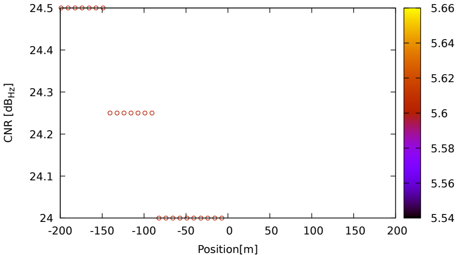
CNR vs position for C02 (B1) on Xiaomi11T - DOY 263 jam. 1
