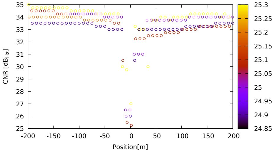
CNR vs position for C16 (B1) on Xiaomi11T - DOY 263 jam. 1
