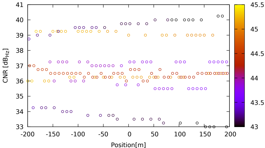
CNR vs position for C21 (B1) on Xiaomi11T - DOY 263 jam. 2
