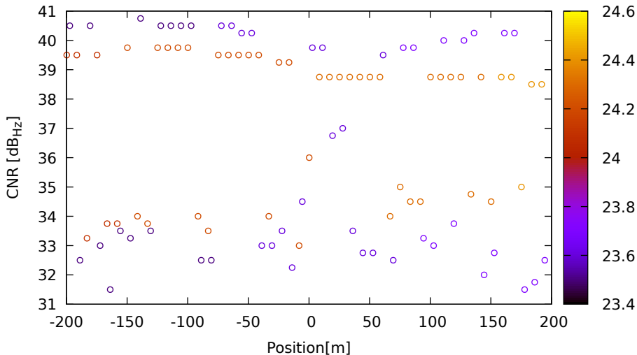
CNR vs position for C28 (B1) on Xiaomi11T - DOY 263 jam. 3
