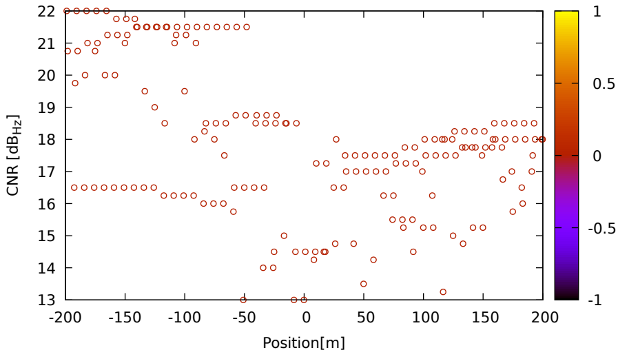
CNR vs position for E02 (E5a) on Xiaomi11T - DOY 263 jam. 1
