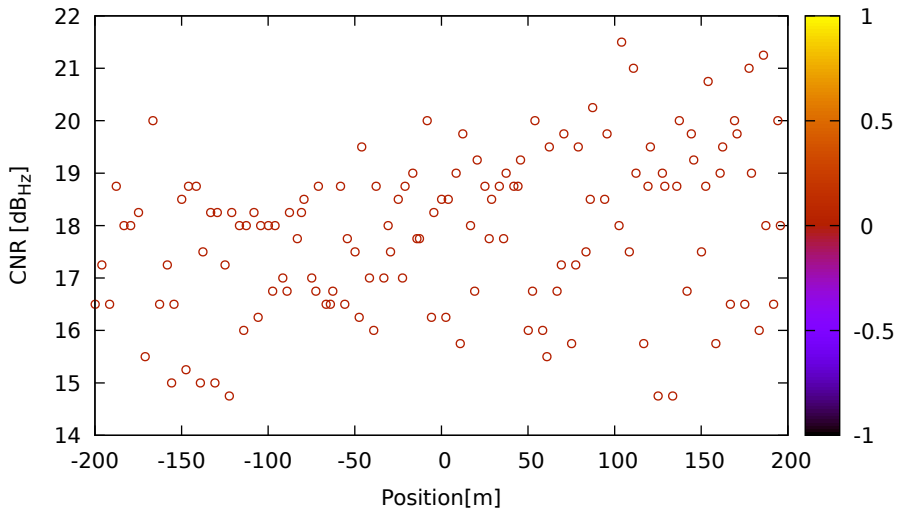
CNR vs position for E02 (E5a) on Xiaomi11T - DOY 263 jam. 2
