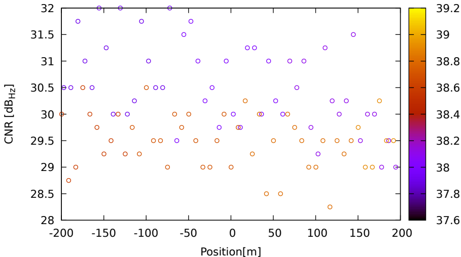
CNR vs position for E04 (E5a) on Xiaomi11T - DOY 263 jam. 3
