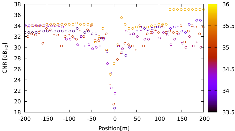
CNR vs position for E11 (E1) on Xiaomi11T - DOY 263 jam. 1
