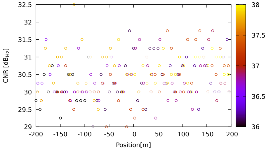
CNR vs position for E11 (E5a) on Xiaomi11T - DOY 263 jam. 2
