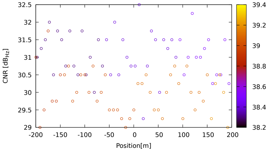
CNR vs position for E11 (E5a) on Xiaomi11T - DOY 263 jam. 3
