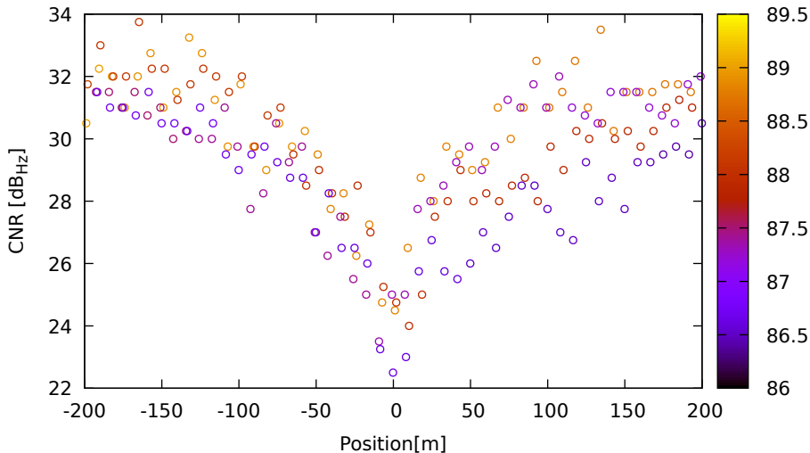
CNR vs position for E12 (E5a) on Xiaomi11T - DOY 263 jam. 1
