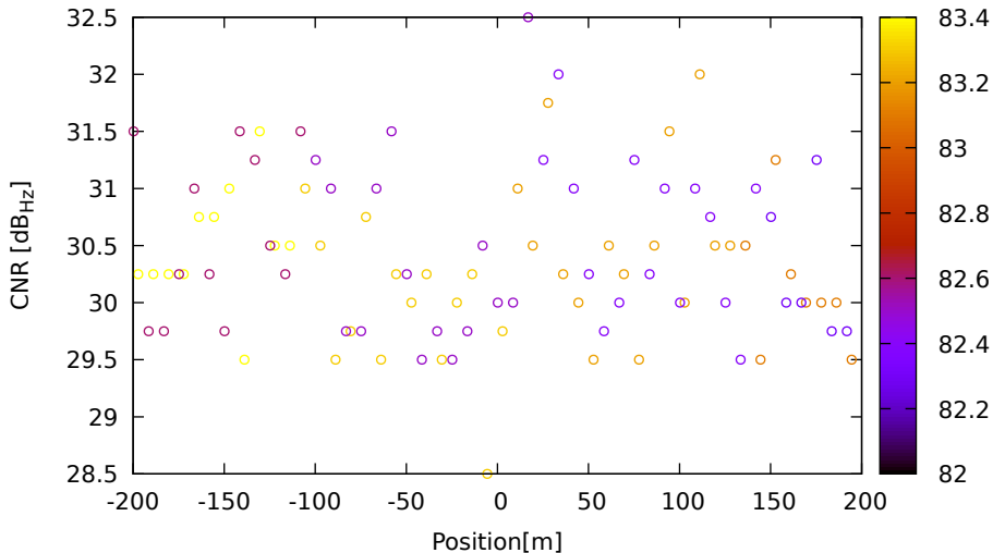
CNR vs position for E12 (E5a) on Xiaomi11T - DOY 263 jam. 3
