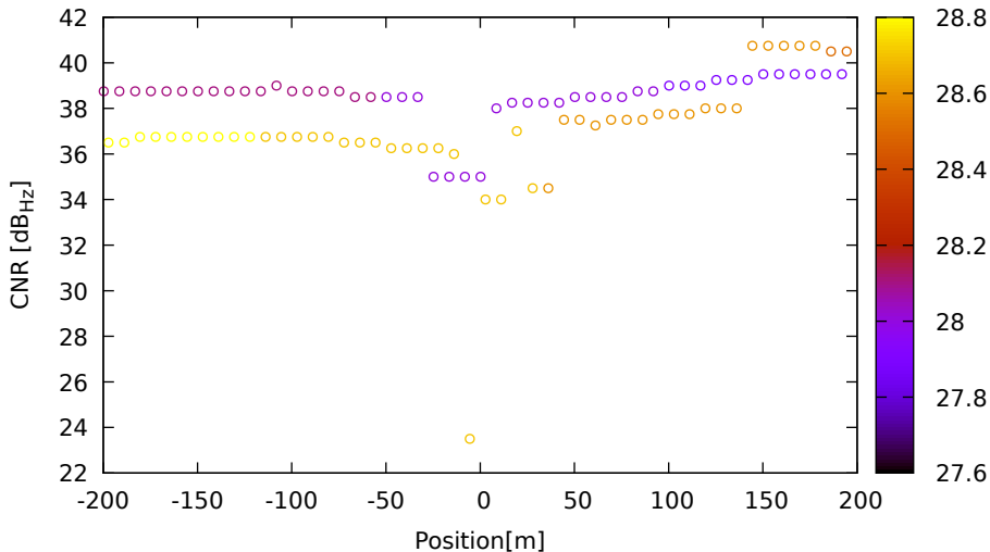
CNR vs position for E33 (E1) on Xiaomi11T - DOY 263 jam. 3
