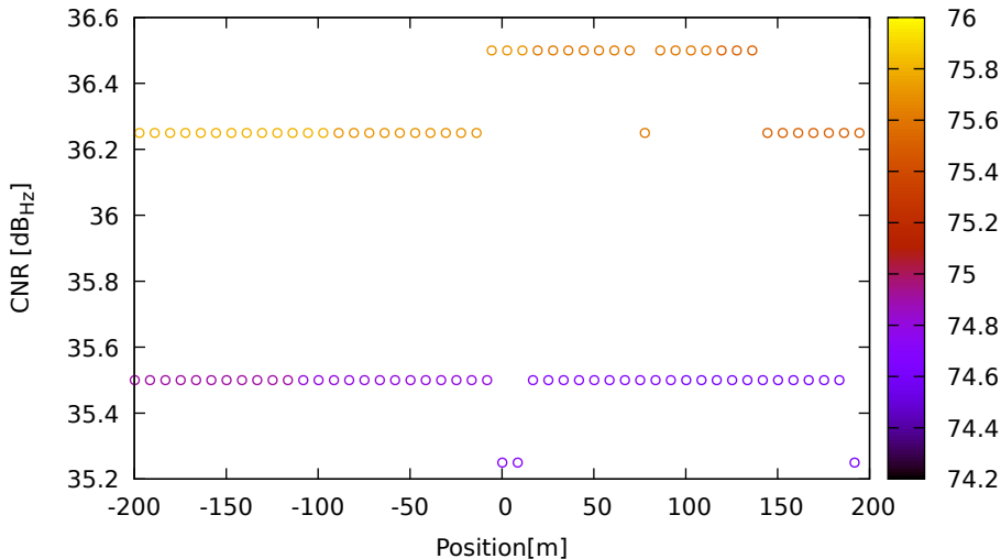
CNR vs position for G01 (L5) on Xiaomi11T - DOY 263 jam. 3
