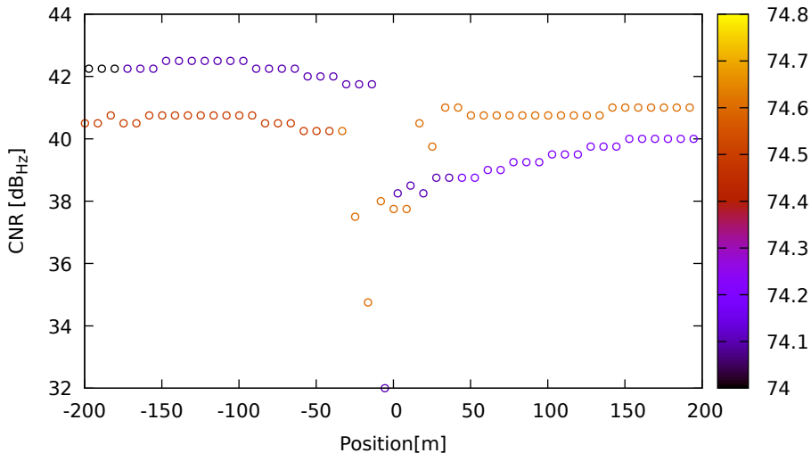
CNR vs position for G03 (L1) on Xiaomi11T - DOY 263 jam. 3
