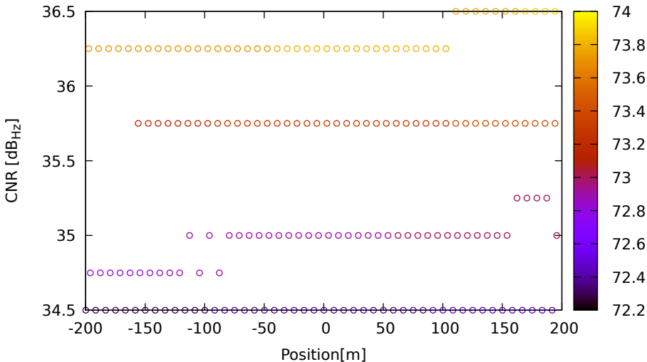
CNR vs position for G03 (L5) on Xiaomi11T - DOY 263 jam. 2
