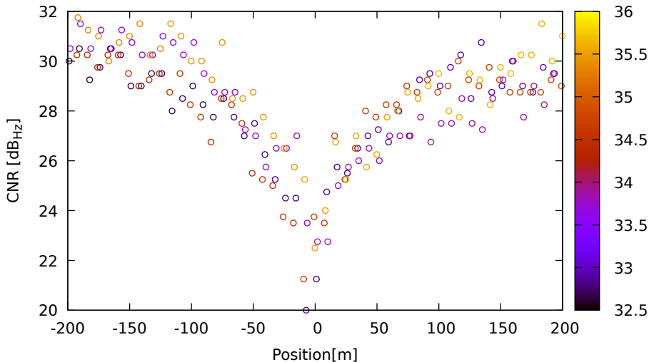
CNR vs position for G04 (L5) on Xiaomi11T - DOY 263 jam. 1
