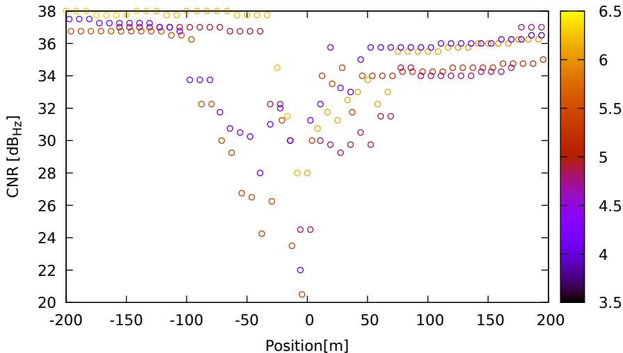
CNR vs position for G08 (L1) on Xiaomi11T - DOY 263 jam. 2
