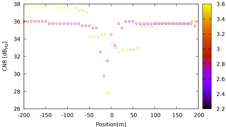
CNR vs position for G08 (L1) on Xiaomi11T - DOY 263 jam. 3
