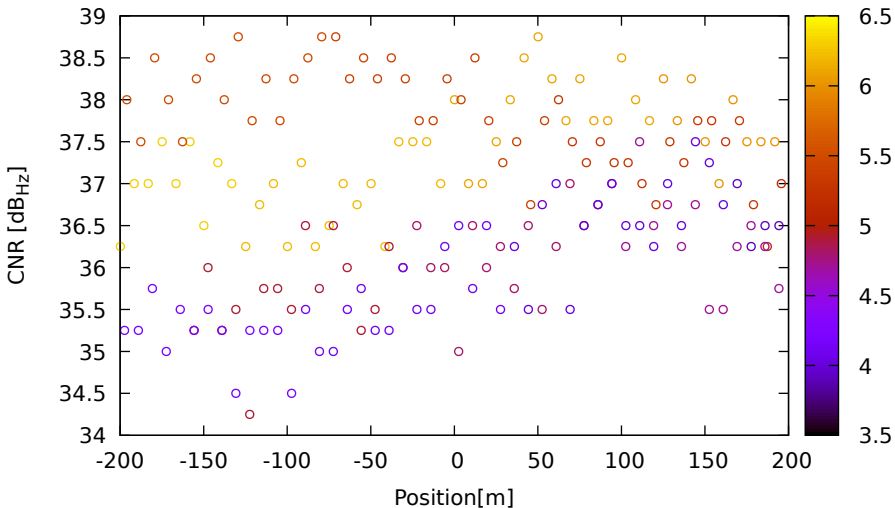
CNR vs position for G08 (L5) on Xiaomi11T - DOY 263 jam. 2
