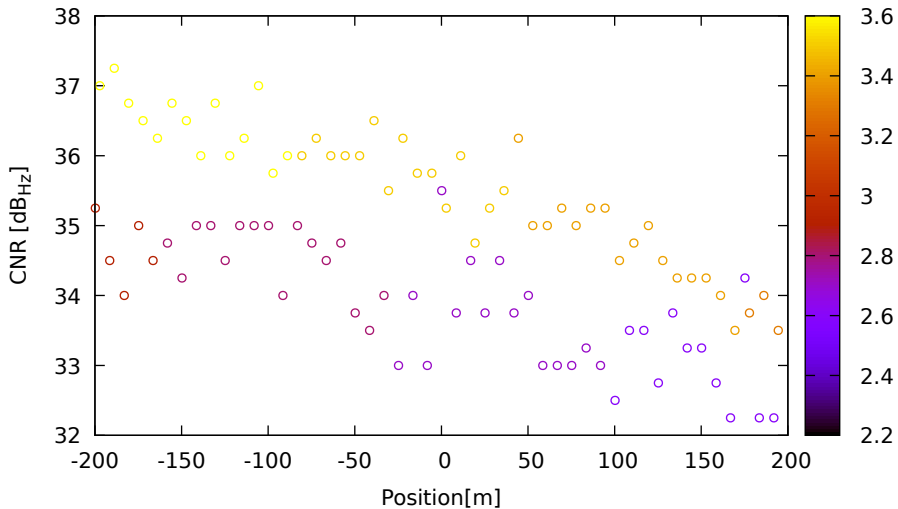
CNR vs position for G08 (L5) on Xiaomi11T - DOY 263 jam. 3
