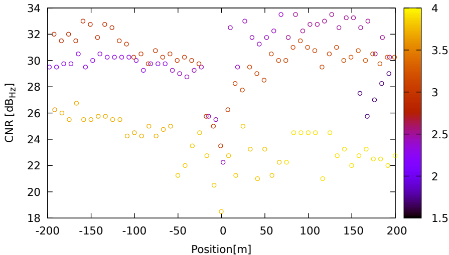
CNR vs position for G09 (L1) on Xiaomi11T - DOY 263 jam. 1
