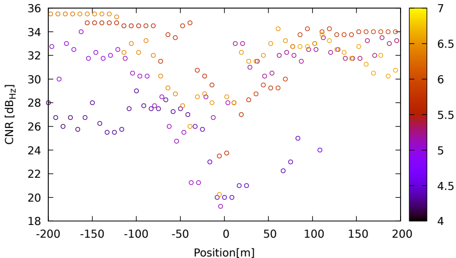
CNR vs position for G09 (L1) on Xiaomi11T - DOY 263 jam. 2
