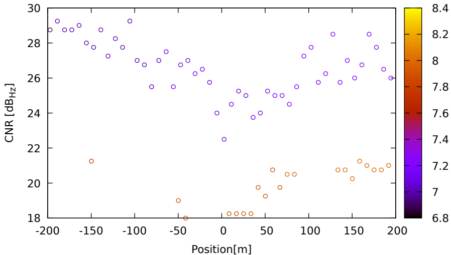
CNR vs position for G09 (L1) on Xiaomi11T - DOY 263 jam. 3
