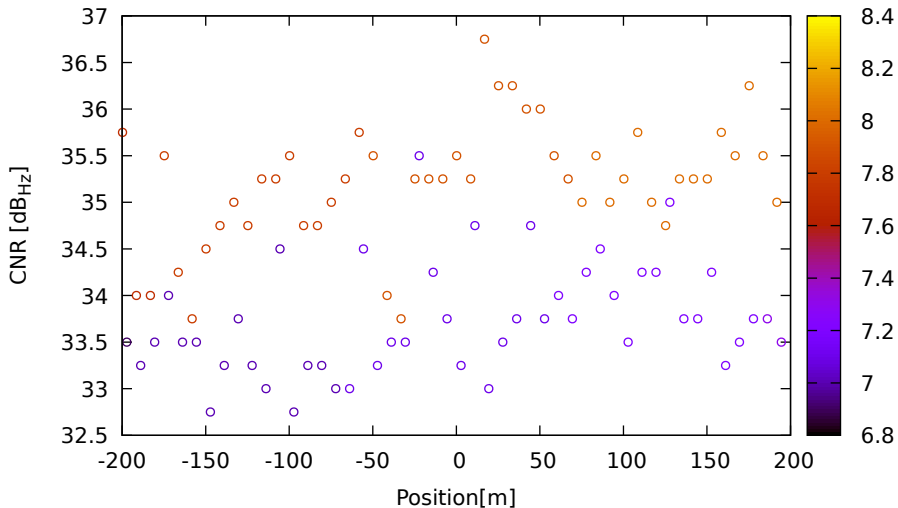
CNR vs position for G09 (L5) on Xiaomi11T - DOY 263 jam. 3
