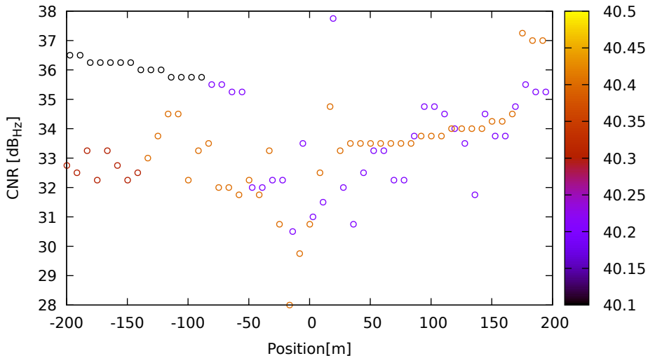
CNR vs position for G17 (L1) on Xiaomi11T - DOY 263 jam. 3
