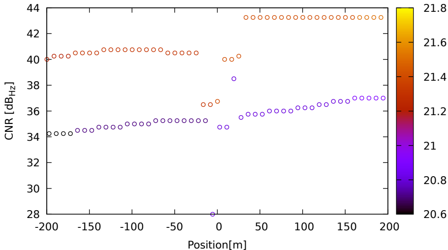
CNR vs position for G19 (L1) on Xiaomi11T - DOY 263 jam. 3
