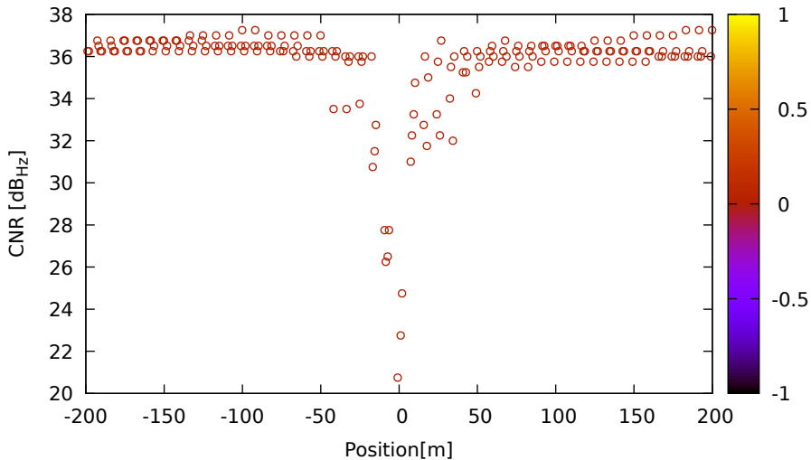
CNR vs position for G28 (L1) on Xiaomi11T - DOY 263 jam. 1
