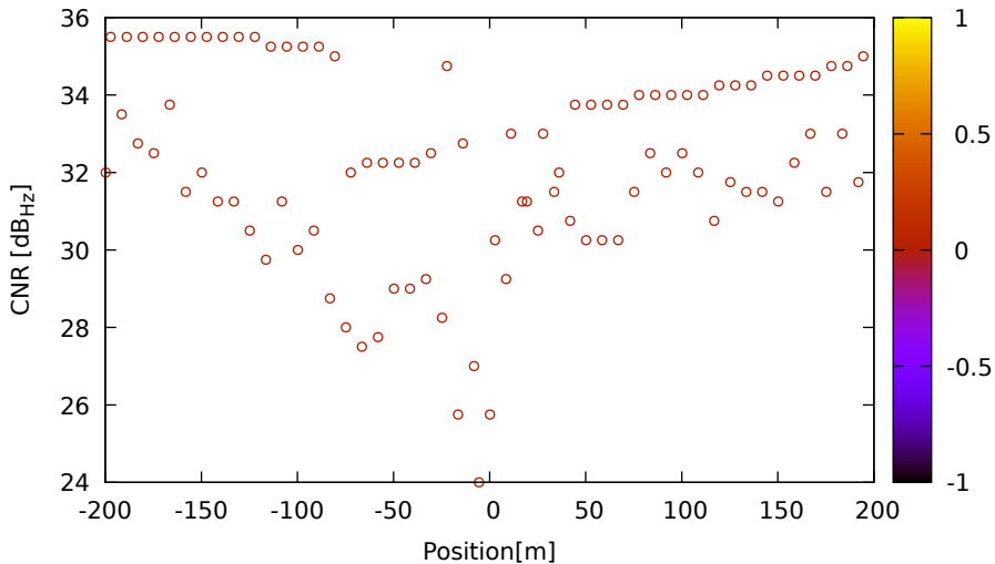
CNR vs position for G28 (L1) on Xiaomi11T - DOY 263 jam. 3
