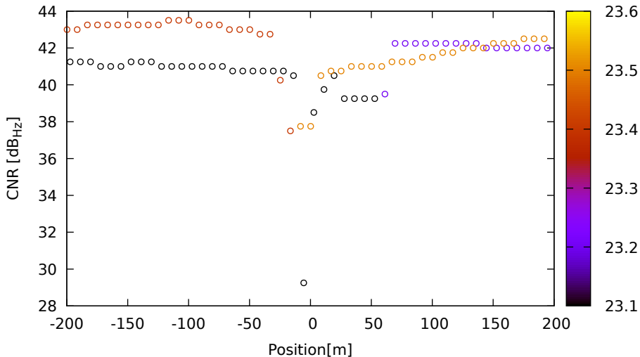
CNR vs position for G31 (L1) on Xiaomi11T - DOY 263 jam. 3
