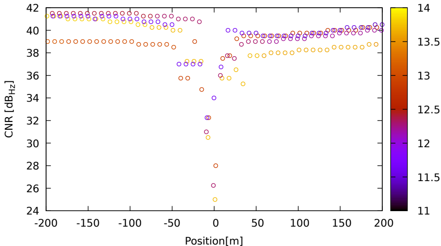
CNR vs position for G32 (L1) on Xiaomi11T - DOY 263 jam. 1
