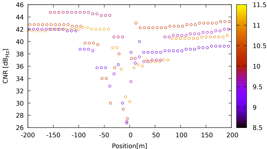
CNR vs position for G32 (L1) on Xiaomi11T - DOY 263 jam. 2
