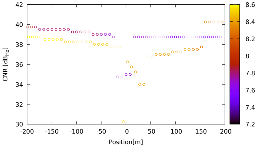
CNR vs position for G32 (L1) on Xiaomi11T - DOY 263 jam. 3
