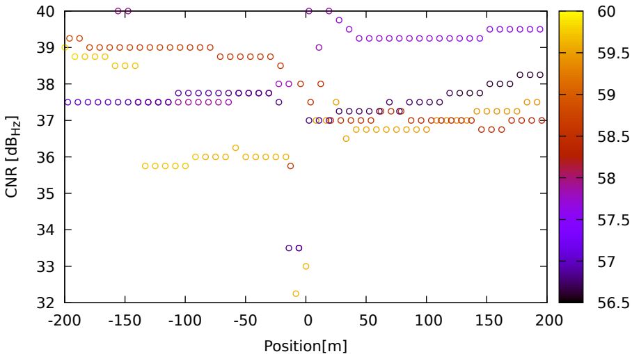
CNR vs position for R01 (G1) on Xiaomi11T - DOY 263 jam. 2
