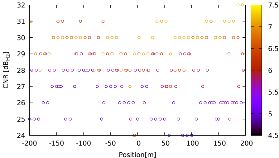
CNR vs position for R03 (G1) on Xiaomi11T - DOY 263 jam. 2
