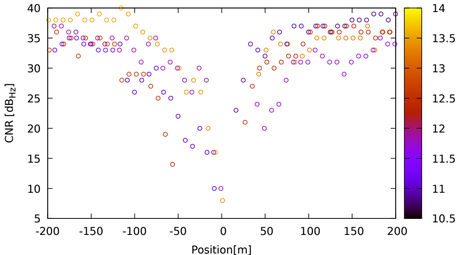
CNR vs position for R08 (G1) on Xiaomi11T - DOY 263 jam. 1
