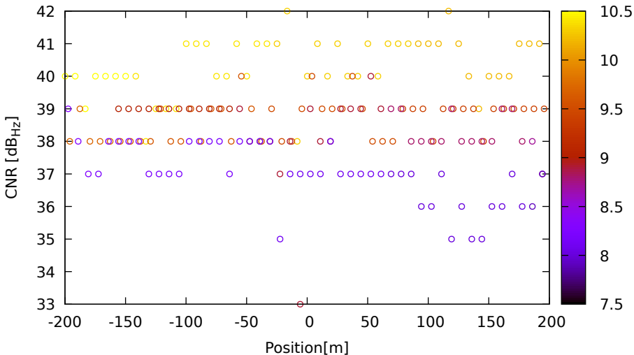
CNR vs position for R08 (G1) on Xiaomi11T - DOY 263 jam. 2
