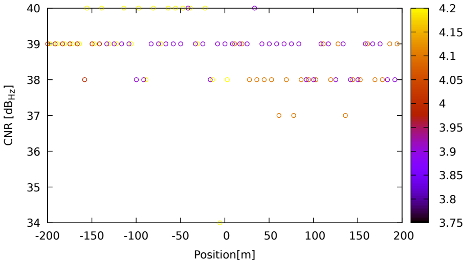
CNR vs position for R09 (G1) on Xiaomi11T - DOY 263 jam. 3
