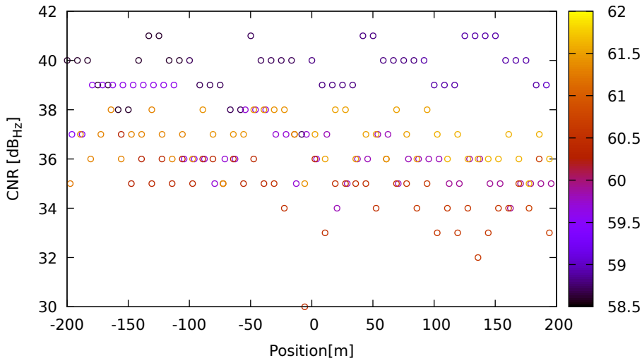
CNR vs position for R17 (G1) on Xiaomi11T - DOY 263 jam. 2
