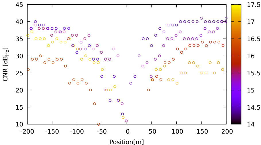
CNR vs position for R23 (G1) on Xiaomi11T - DOY 263 jam. 1
