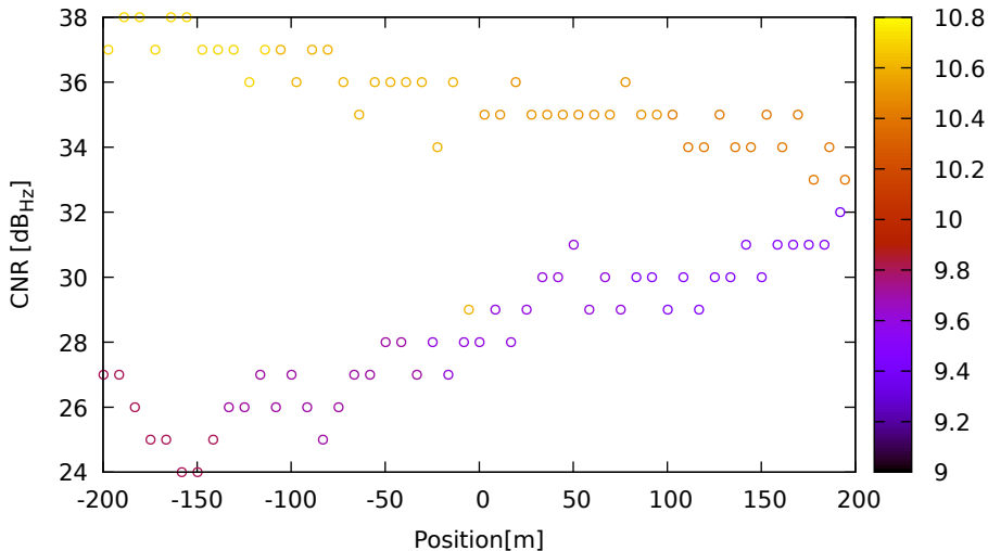
CNR vs position for R23 (G1) on Xiaomi11T - DOY 263 jam. 3
