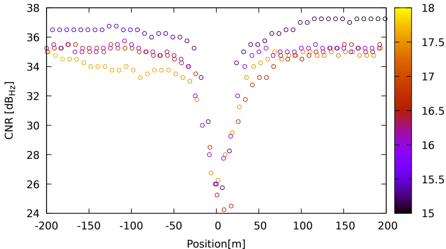
CNR vs position for C12 (B1) on XiaomiMi8 - DOY 263 jam. 1
